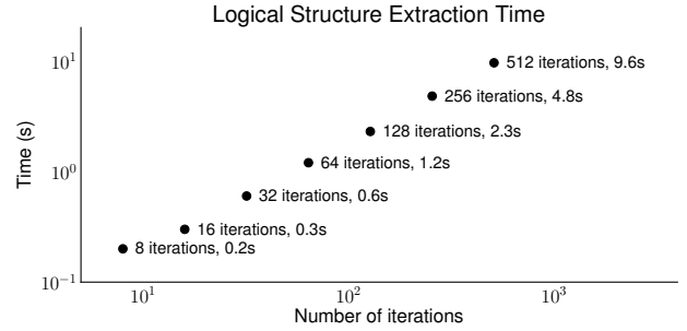
Figure 18: Time to calculate logical structure for a 64-char LULESH execution at increasing iterations.
