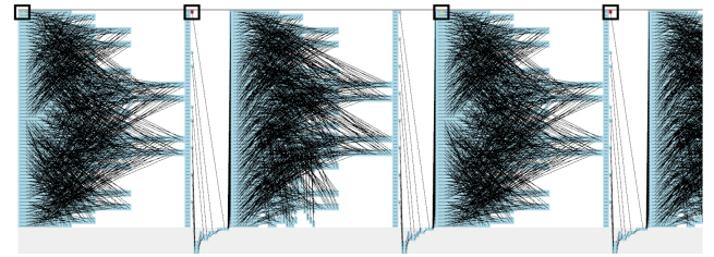
Figure 22: 64-char LASSEN trace colored by differential duration. Like Figure 21, the logical structure shows repeated long events (boxed) over iterations.
