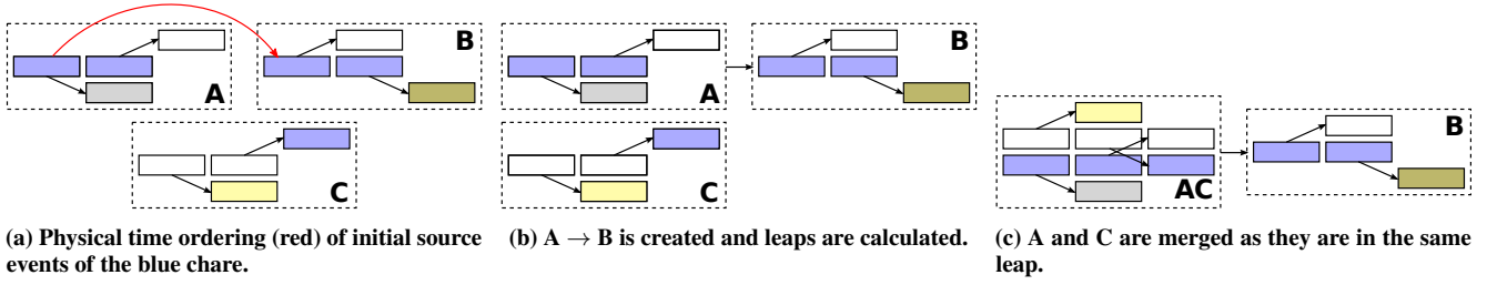
Figure 5: We infer happened-before relationships using physical time between initial source events within partitions. We merge partitions at the same leap with overlapping chares. Event color indicates chore.
