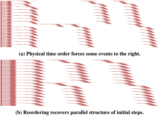
Figure 10: Logical structures of a traced 1,024-process MPI merge tree algorithm. Irregular receive order forces some events to be stepped much later than their peers. Reordering restores regularity.
