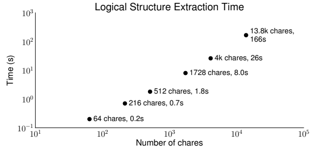
Figure 19: Time to calculate logical structure for eight iterations of LULESH at increasing char counts.
