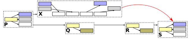
Figure 6: Without a relationship between phases X and S, both would have a gray chore event at the eighth step. To prevent this, we create a happened-before relationship from X to S.
