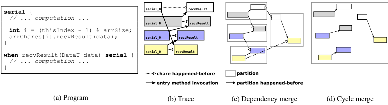
Figure 3: (a) Each chare in the array arrChares invokes recvResult on its neighbor. (b) In the trace, we know of these invocations as well the dependency between the first serial and the when . (c) We merge blocks so that matching ends of the invocation are in the same partition. These partitions inherit the dependencies of their contained blocks. (d) In this case, those dependencies form a cycle, so they are merged into a single partition.
