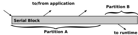
Figure 2: Initial partitions can contain sequences of dependency events within a serial block. Partition boundaries are made when the dependencies cross application-runtime boundaries.
