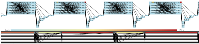
Figure 21: 8-char LASSEN trace colored by differential duration. In the logical structure (top), a repeated pattern shows the same events of the same chare are associated with higher duration. Physical time (bottom) makes it difficult to discern these events are the same, as there is no indication where it falls in the control flow.
