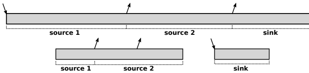
Figure 13: Three examples showing how serial blocks are divided based on the dependency events.
